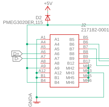
USB TYPE C CONNECTOR
